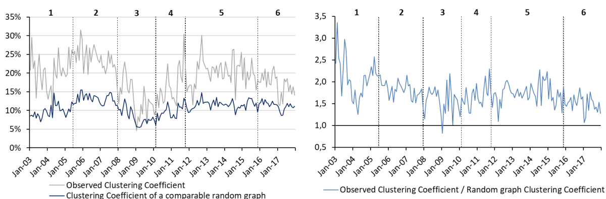
Figure 12 | Clustering coefficient
